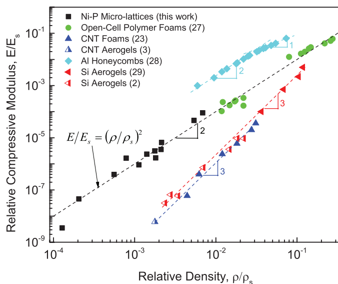
Fig. 4. Relative compressive modulus (defined as the measured Young’s modulus, E , divided by the Young’s modulus of the constituent solid, E_s ) of selected cellular materials at low relative density.
